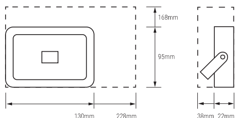
ASTRID HIGHLITE ECO
